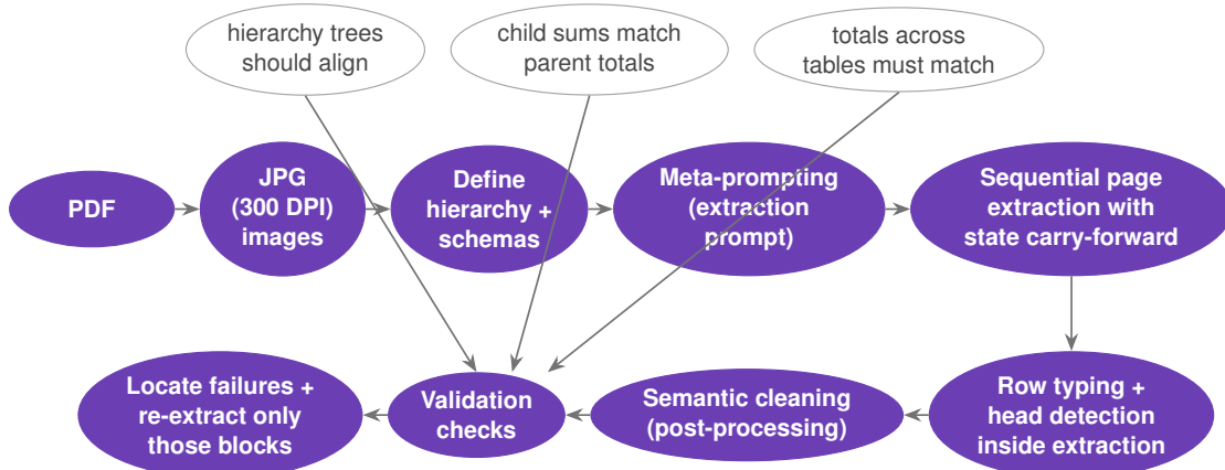
Figure 3.2: Tab2DB — the actual nine-stage implemented pipeline with multi-level validation and selective re-extraction
