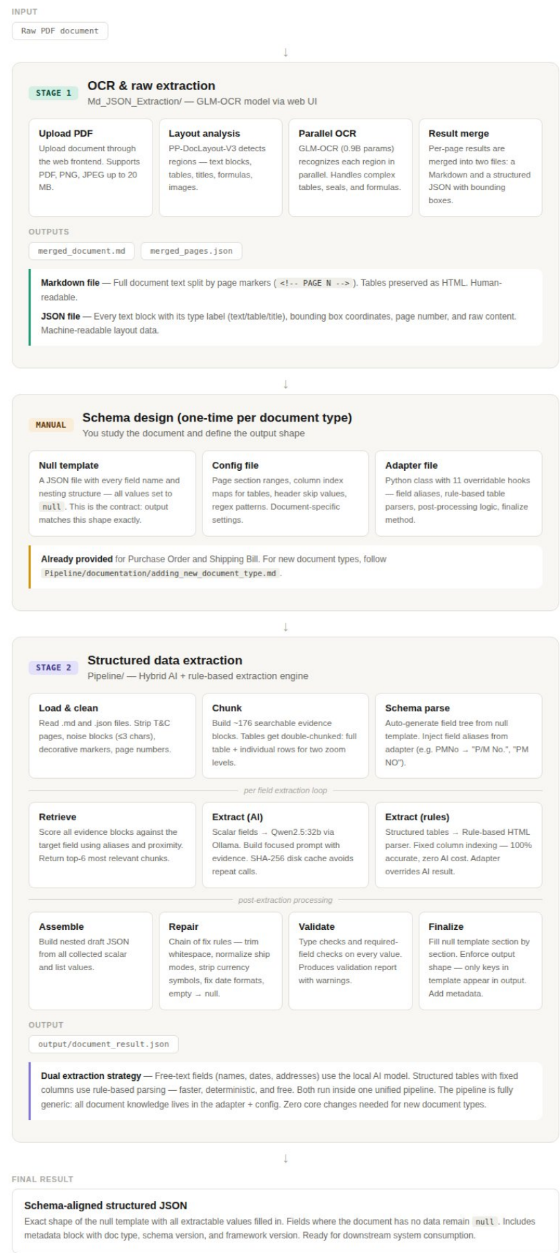
19 Figure 4.1: Final pipeline workflow — Stage 1 OCR & raw extraction, manual schema design, and Stage 2 structured data extraction (top to bottom)
