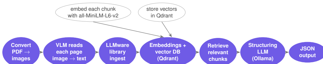
Figure 3.3: LLMware — the actual seven-stage implemented pipeline with separate embedding, vector store, and retrieval components
